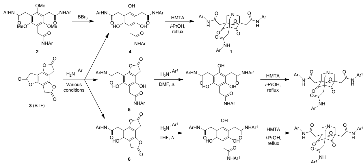
Figure 2. Ring opening of BTF ( 3 ) to form phloroglucinol derivatives ( 4 ) provides a much milder route to aryl amide AATs ( 1 ) than previous (1, 12) BBr_3 deprotection procedures ( Ar = aryl ), and opportunities to rationally prepare non- C_3 -symmetric derivatives. HMTA = hexamethylenetetramine.
