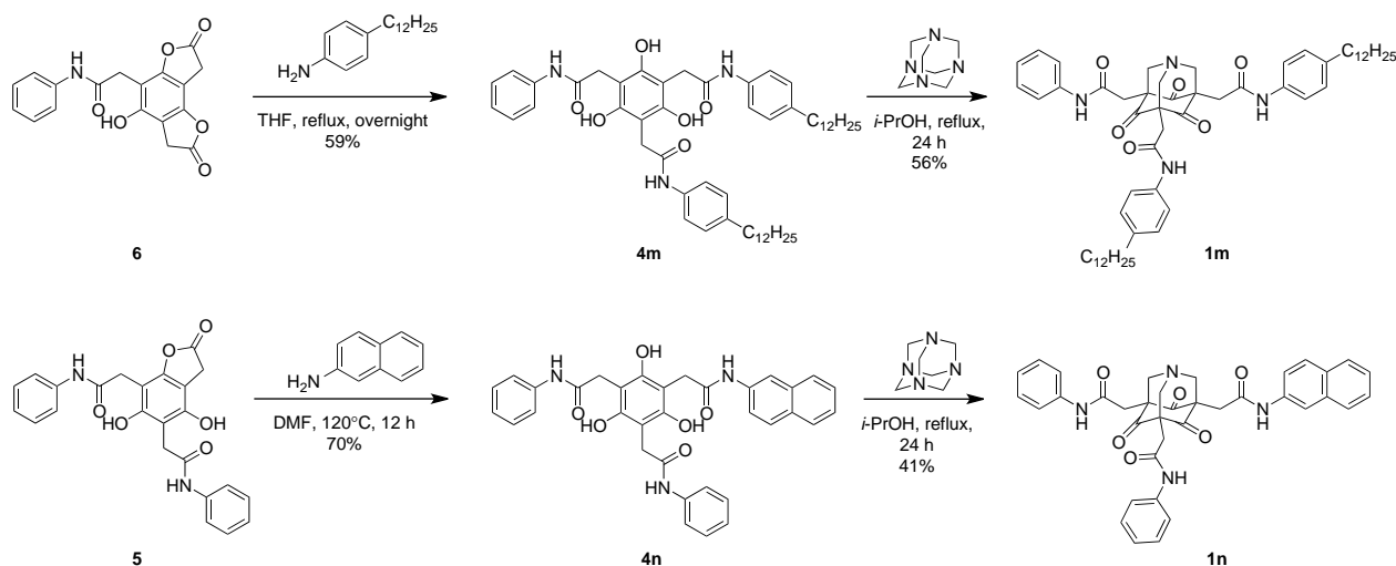
Figure 4. Utilisation of 5 and 6 for the synthesis of C_3 -symmetric AAT molecules.
