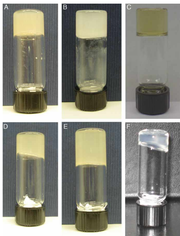
Figure 5. Inverted gels formed in sealed glass vials. (A) 0.30 wt% compound 1e in \text{CHCl}_3 , (B) 0.30 wt% compound 1g in TCE, (C) 0.20 wt% compound 1j in toluene, (D) 0.30 wt% of an equimolar 1e and 1g in TCE, (E) 0.25 wt% equimolar amounts of 1e and 1g in a 2:1 mixture of \text{CHCl}_3 :TCE and (F) 0.40 wt% compound 1m in \text{CHCl}_3 .
