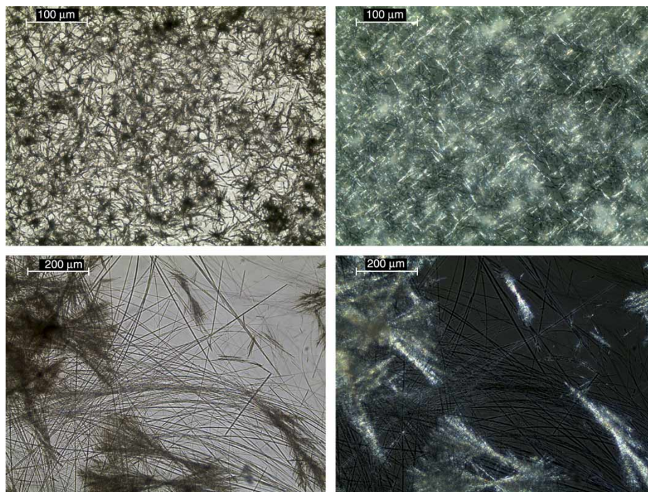
Figure 7. POM images of the native gel phases (top row is 1e in \text{CHCl}_3 ; bottom row is 1g in TCE; the images on the right side have been taken with the polarisers crossed). Notice the distinctly different morphologies found in the two systems.
